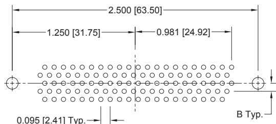
PCDD104 MALE
