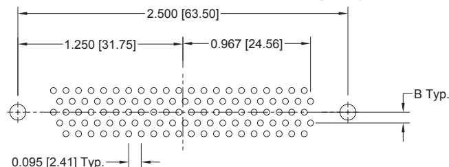
PCDD104 FEMALE
