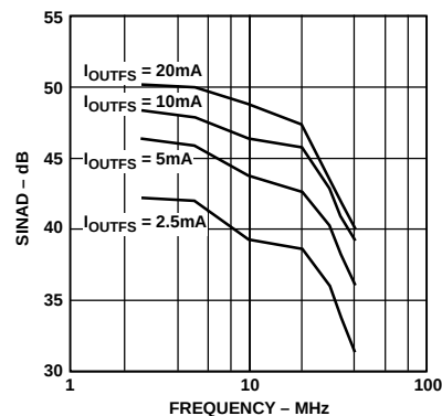
Figure 5. SINAD vs. I_{OUTFS} @ 100 MSPS
