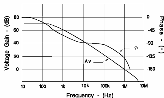
Error Amplifier Open-Loop Frequency Response
