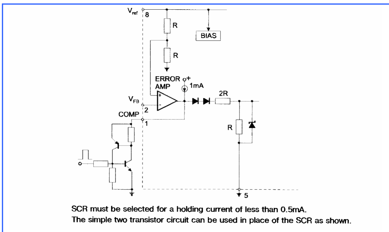
Figure 5:Latched Shutdown
