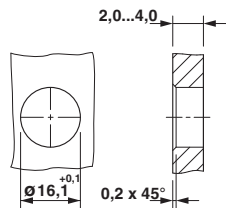
Dimensioned drawing
