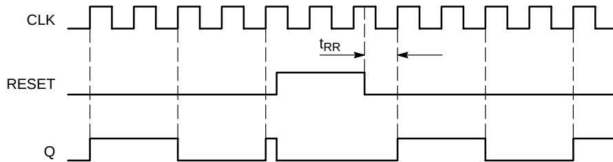
Figure 2. Timing Diagram
