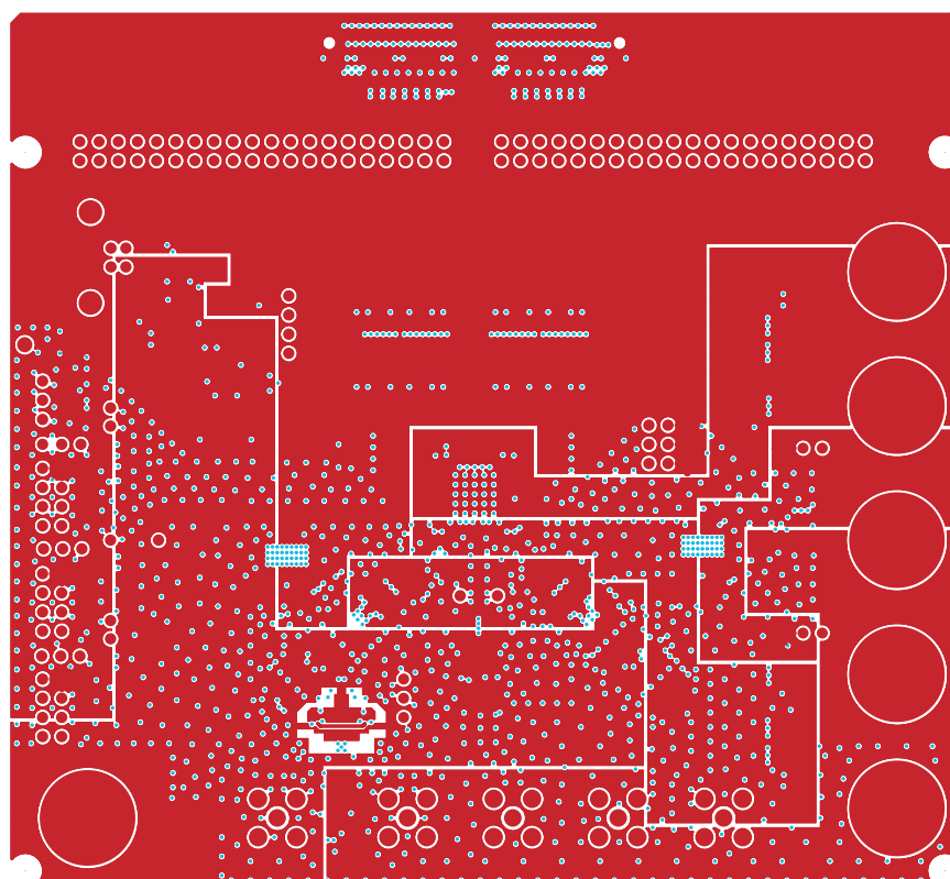
Figure 7. Power Plane 1
