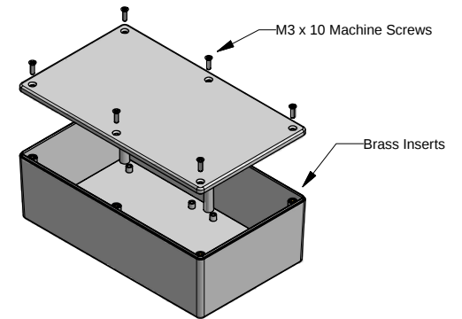
EXPLODED VIEW OF ENCLOSURE
