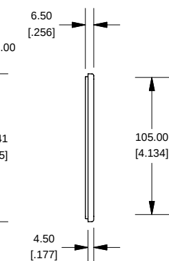
SIDE VIEW OF LID
