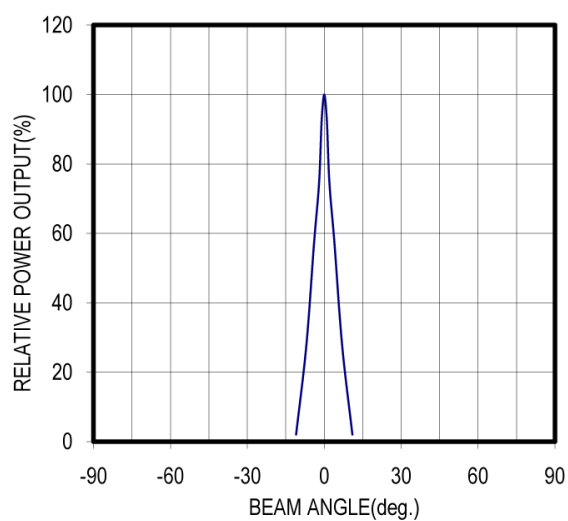
RADIATION PATTERN
