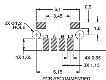
PCB RECOMMENDED
