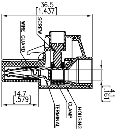
SECTION H-H
