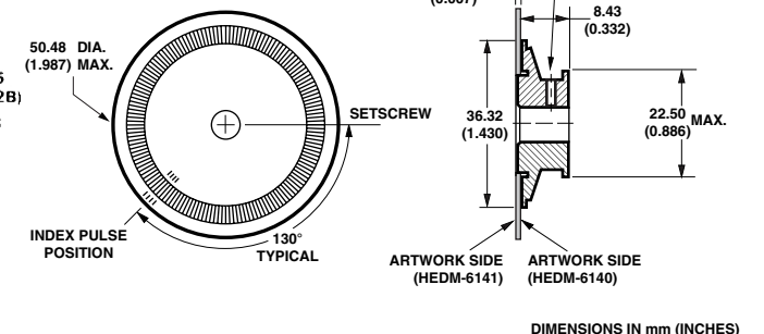
Figure 6b. HEDM-614X Series Codewheel used with HEDS-9040 #T00.
