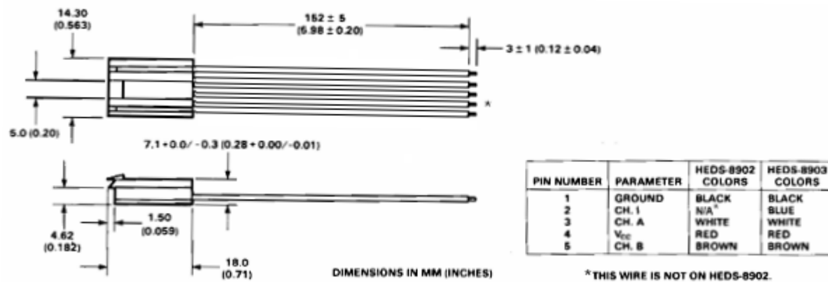
Figure 8. HEDS-8903 Connector.
