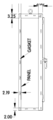
Open End
