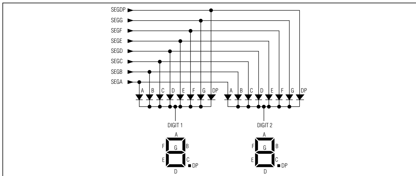
Figure 4. 2-Digit Common-Cathode Configuration
