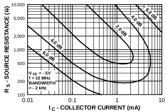
Figure 16. Contours of Constant Narrow Band Noise Figure
