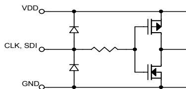
3. CLK, SDI terminal
