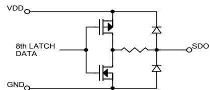
4. SDO terminal
