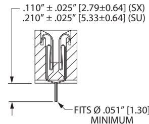
CENTERED DIP SOLDER (SX, SU) AVAILABLE WITH DUAL OR HALF LOADED READOUT TYPE
