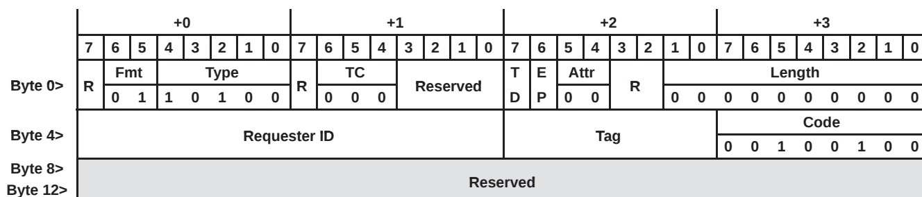
Figure 3–6. PCI Express DEASSERT_INTX Message
