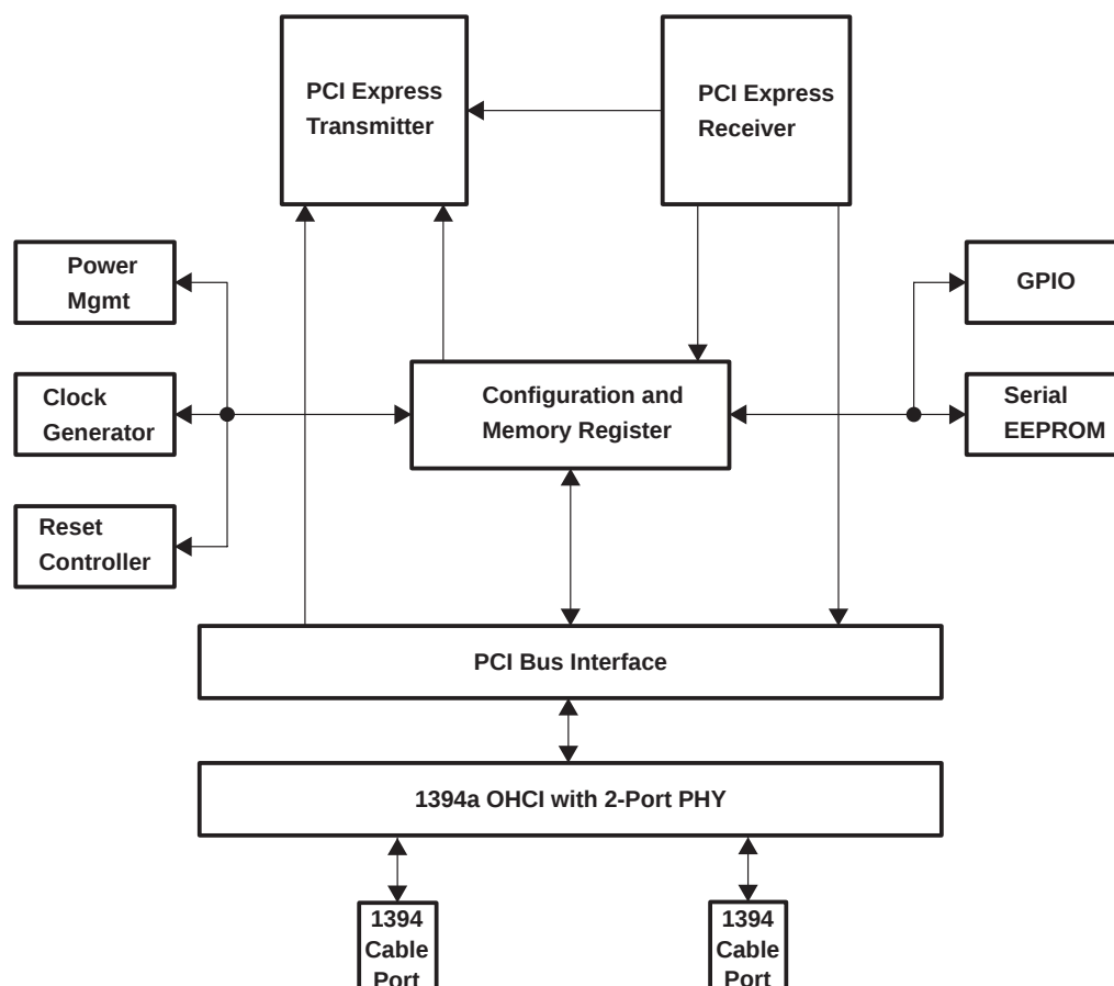
Figure 3–1. XIO2200 Block Diagram
