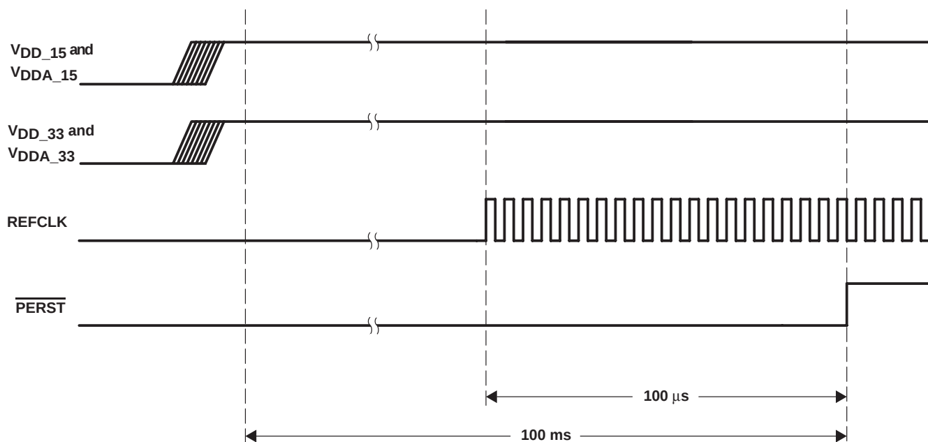
Figure 3–2. Power-Up Sequence
