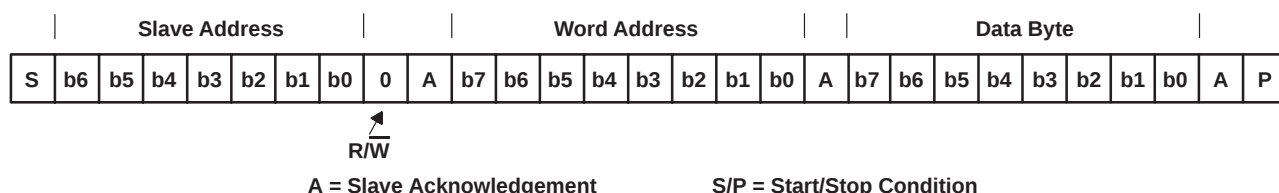
Figure 3–10. Serial-Bus Protocol—Byte Write
