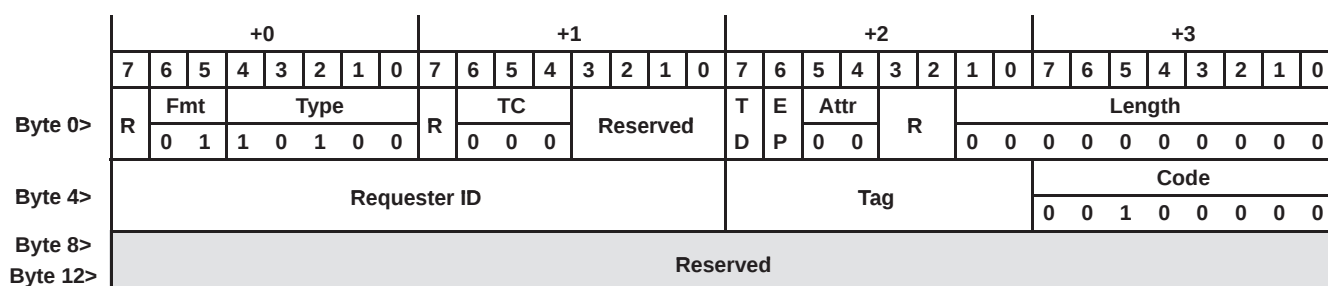
Figure 3–5. PCI Express ASSERT_INTA Message
