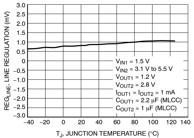
Figure 6. Line Regulation vs. Temperature – V_{OUT} = 2.8 \text{ V}
