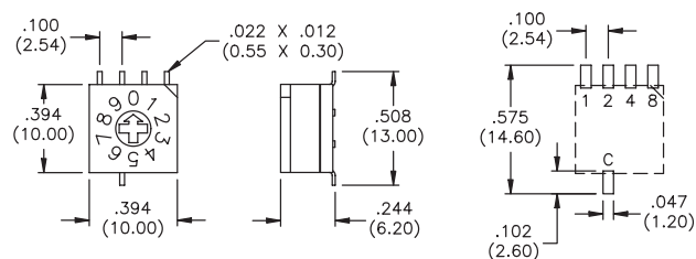
Mechanical outline
