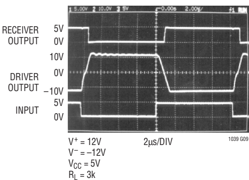
Output Waveforms
