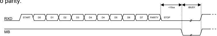
Asynchronous serial communication from host system to VFD module.
