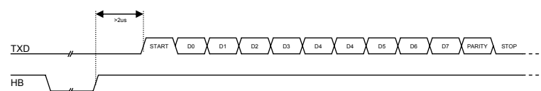
Asynchronous serial communication from VFD module to host system.
