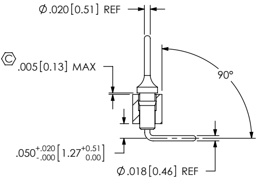
FIG 20 TERMINAL STYLE -N UNLESS OTHERWISE SHOWN, SAME AS FIG1
