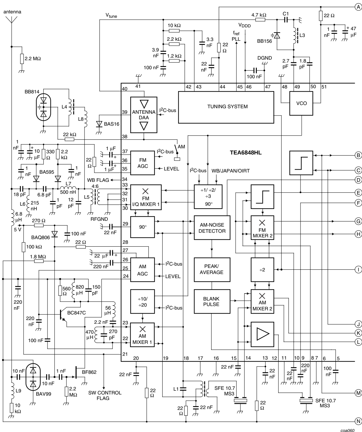
Fig 10. Application diagram (continued in Figure 11)
