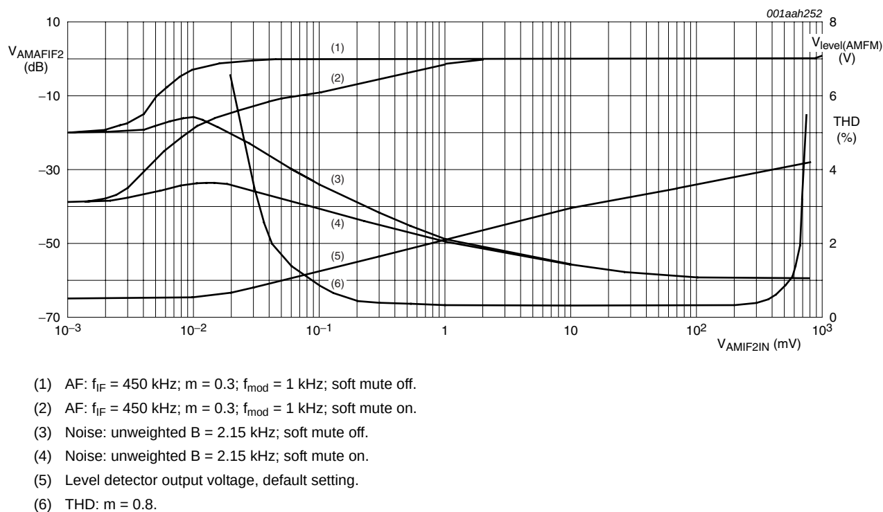
Fig 5. Signal, (S+N)/N, THD and level voltage for AM mode as a function of AMIF2IN voltage
