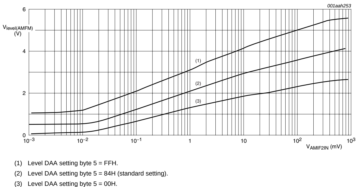
Fig 6. AM level voltage
