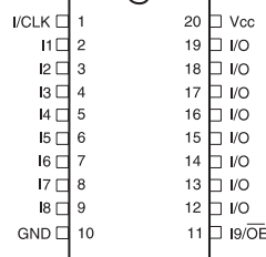
DIP/SOIC
