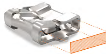
Figure 3. Flared lead-in and milled surface with its low friction make for easier tab insertion.
