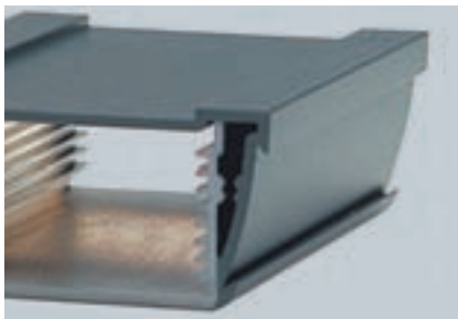
System grooves on the long sides and encapsulated screw channel outside the seal section
