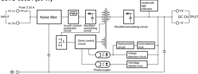
S8VS-03024 (30 W)
