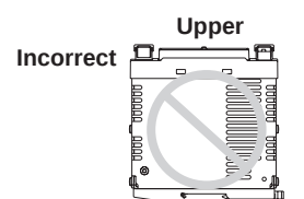
Face-up mounting
