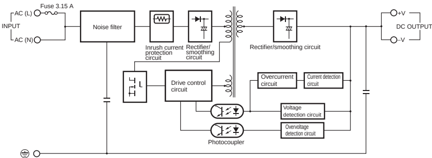
S8VS-06024 (60 W)
