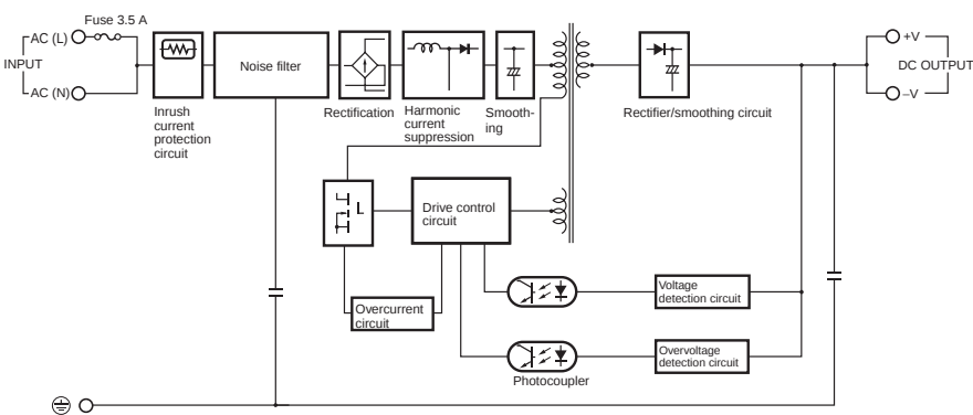
S8VS-12024 (120 W)
