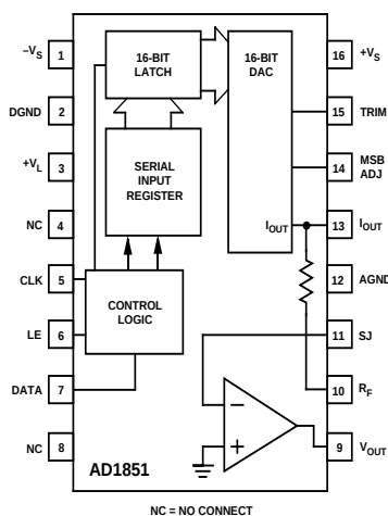
Figure 8a. Schematic Using False Ground
