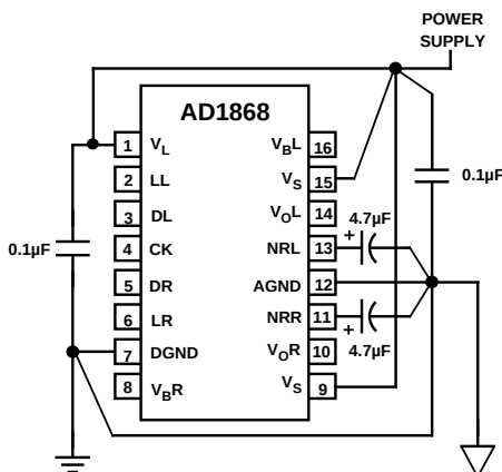
Figure 7. Recommended Circuit Schematic
