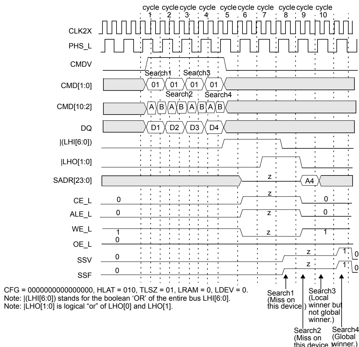
Figure 10-8. Timing Diagram for 72-bit Search Device Number 3 (Last Device)
