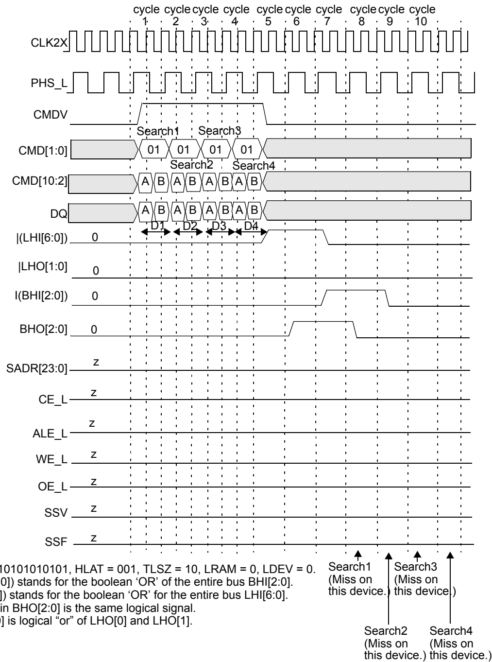
Figure 10-40. Timing Diagram for Devices Below the Winning Device in Block Number 3 Except Device 14 (the Last Device)
