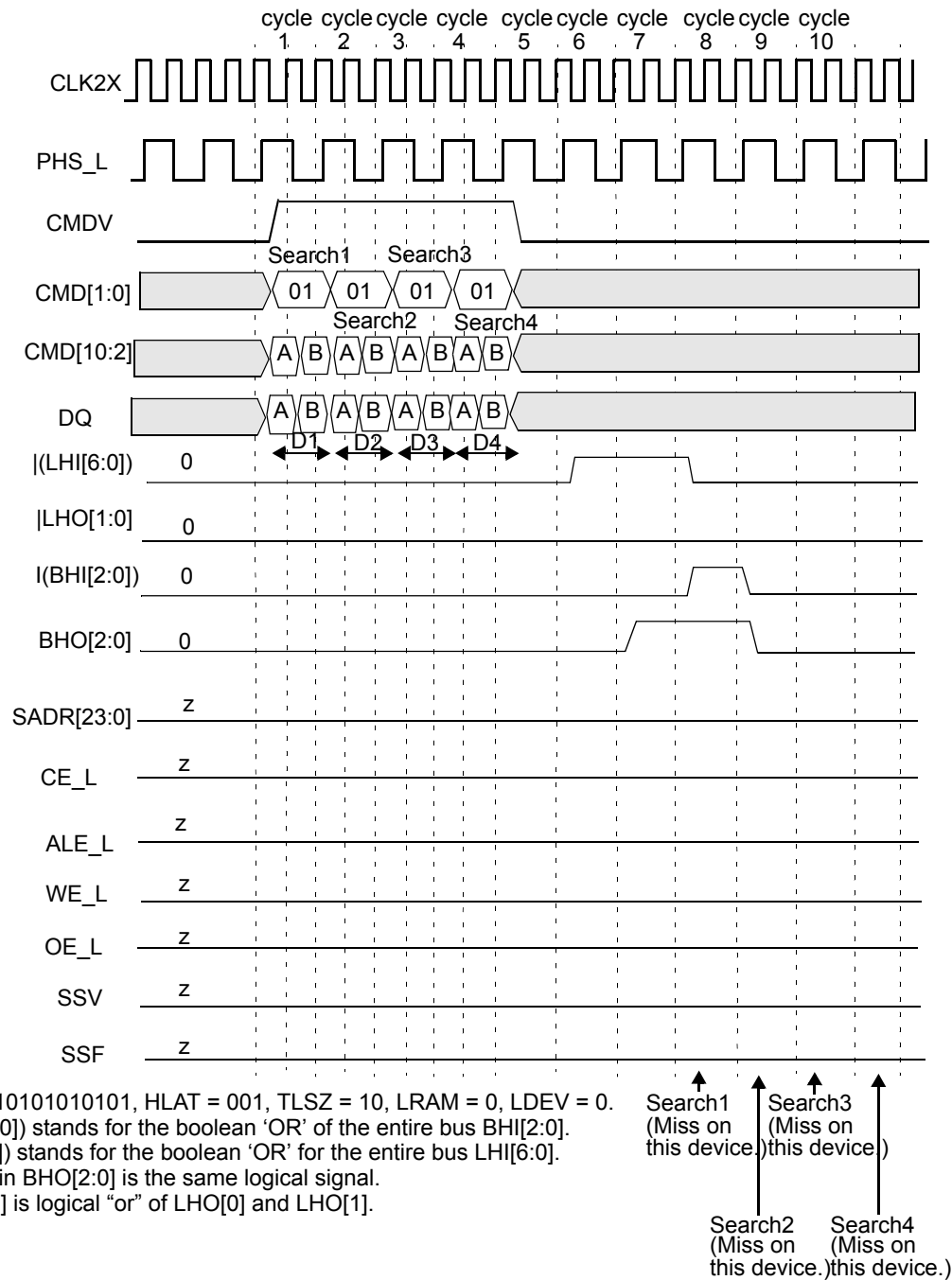
Figure 10-37. Timing Diagram for Devices Below the Winning Device in Block Number 2
