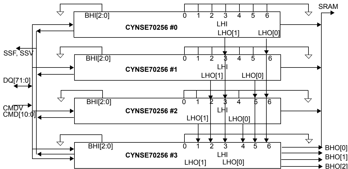
Figure 12-7. Hardware Diagram of a Block of Four Devices
