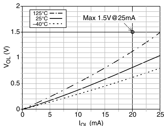
a) V_{\text{DD}} = 5\text{V} , High Drive
