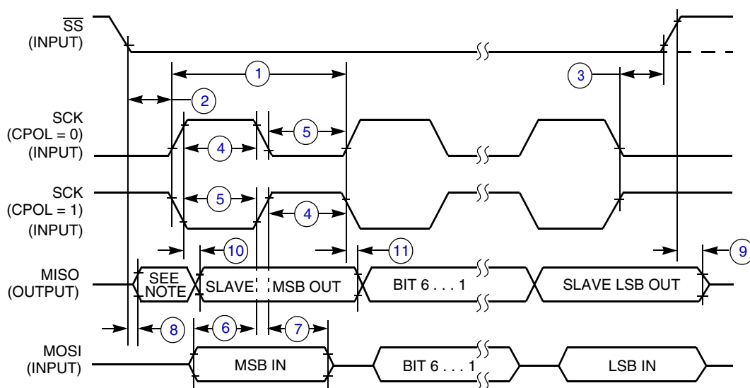
Figure A-17. SPI Slave Timing (CPHA = 1)
