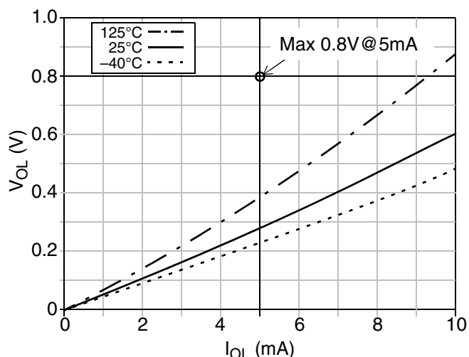
b) V_{\text{DD}} = 3\text{V} , High Drive
