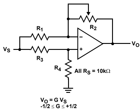
FIGURE 15. ATTENUATOR
