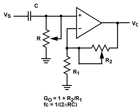
FIGURE 16. FILTER
