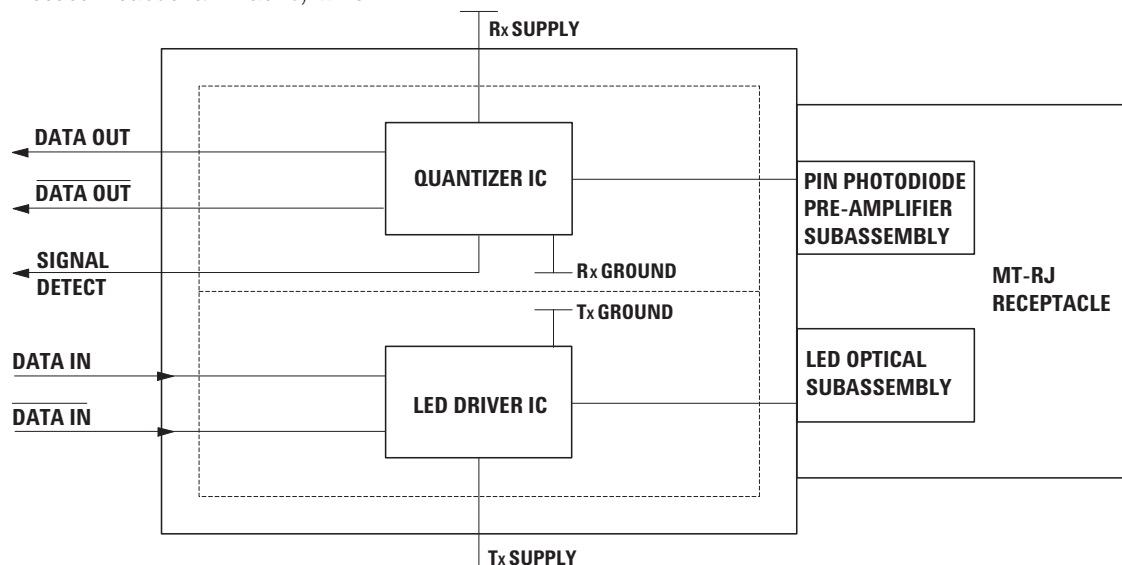
Figure 1. Block Diagram.
