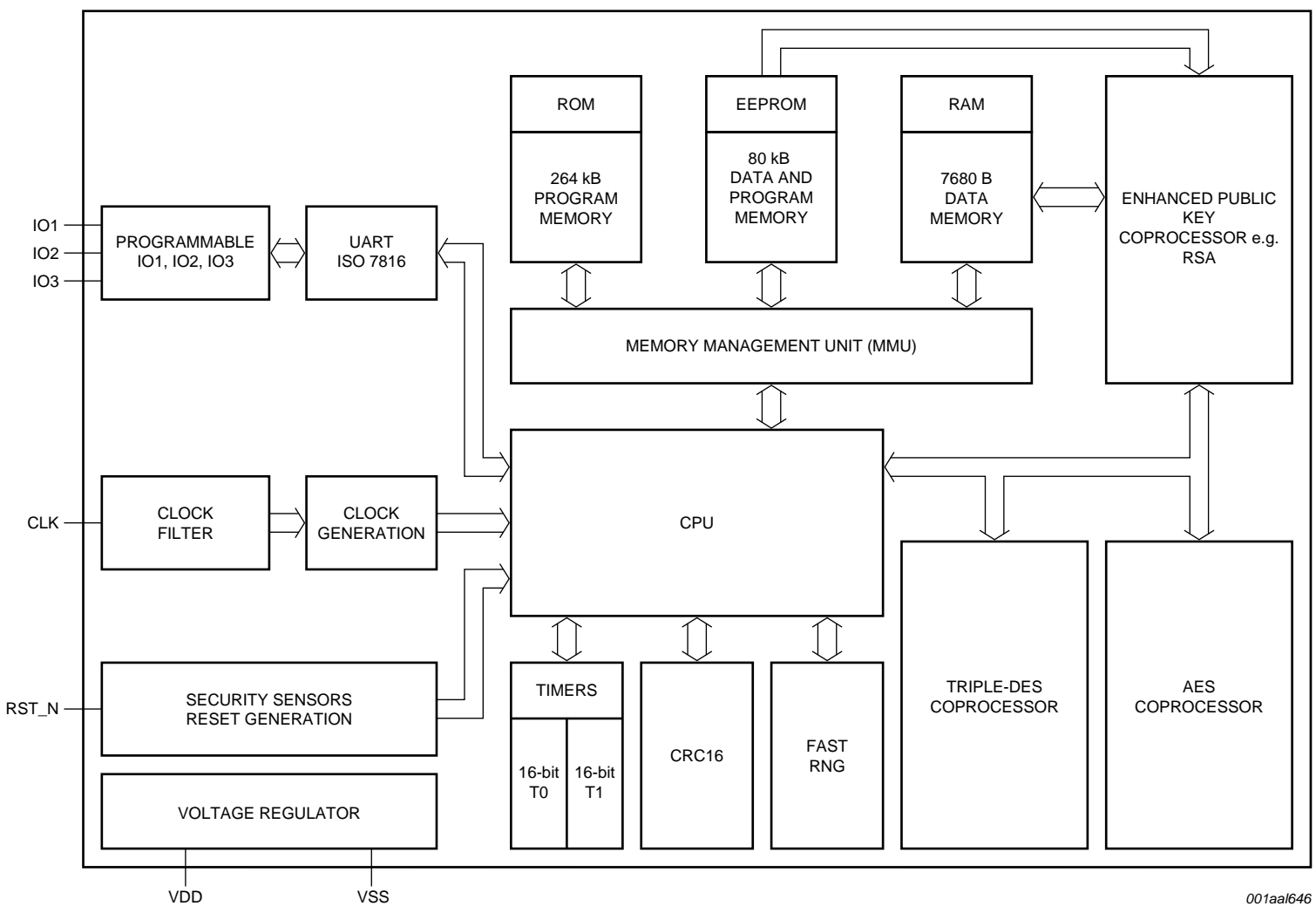
Fig 1. Block diagram
