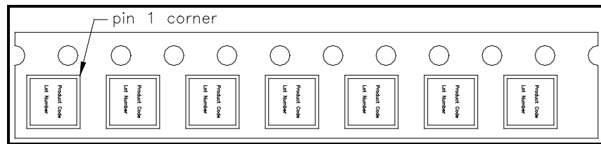
Figure 7: SE5006L-R Tape and Reel Information
