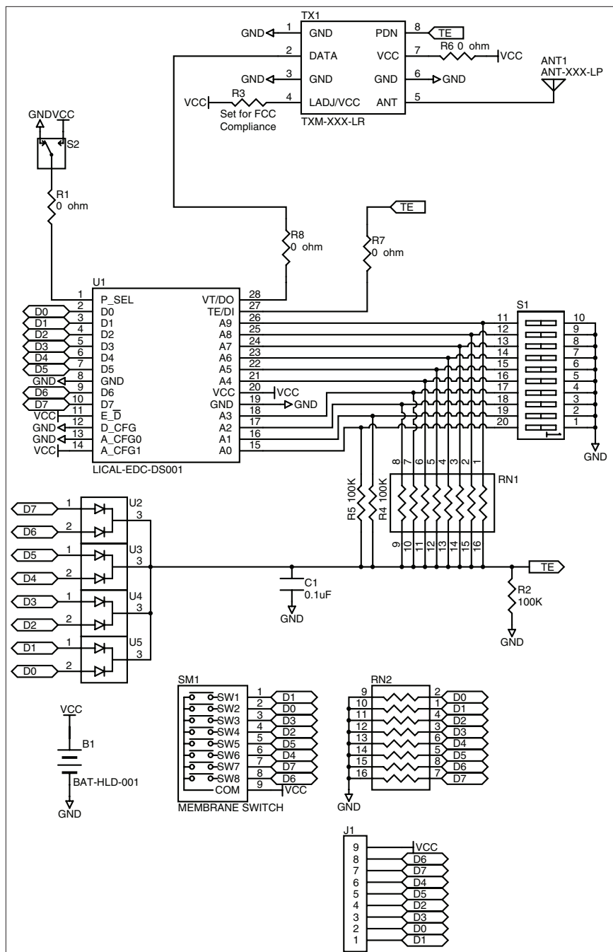
Figure 12: CMD-HHLR-***-MD Schematic
