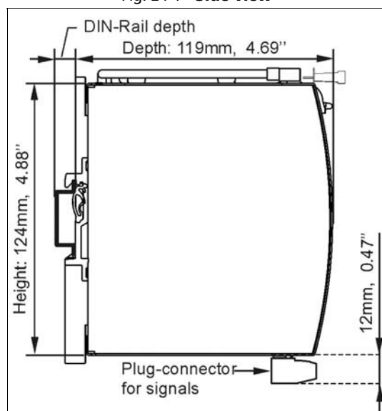
Fig. 24-1 Side view
