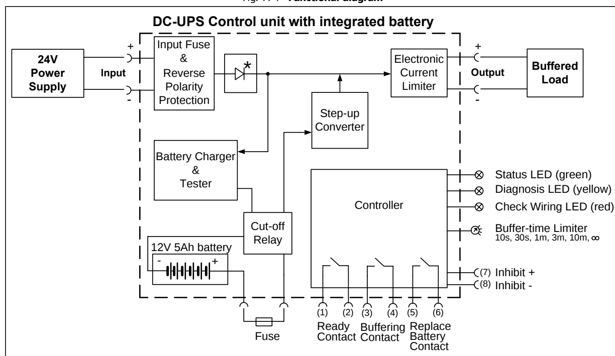
Fig. 11-1 Functional diagram
