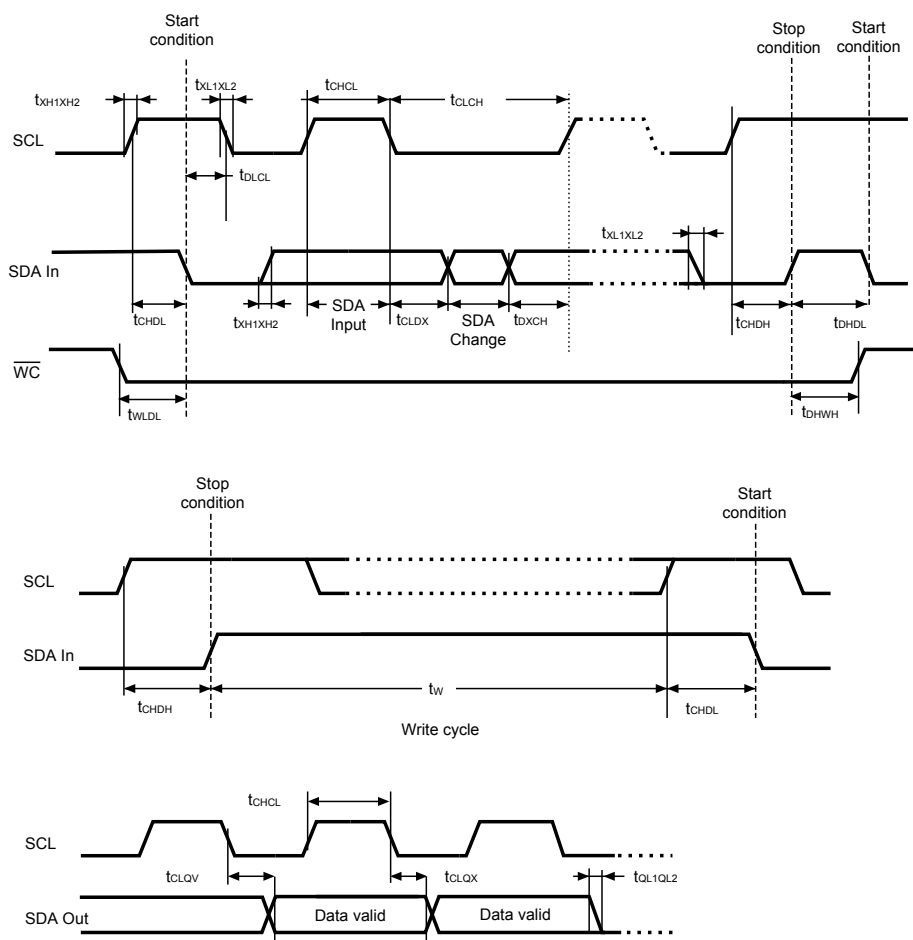
Figure 12. AC waveforms
