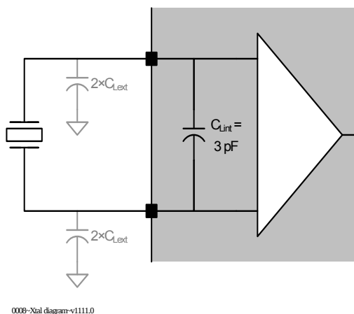
Figure 3-3 • Crystal Oscillator with Optional Additional External Load Capacitors
