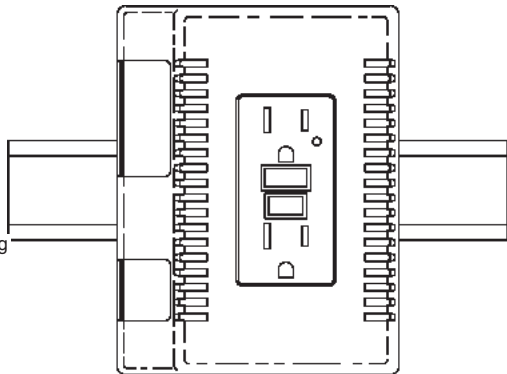
35mm DIN rail mounting foot rotated 90°
