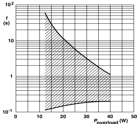
PR01 Time to interruption as a function of overload power for range: 0 R 22 \leq R_n < 1 R 5
