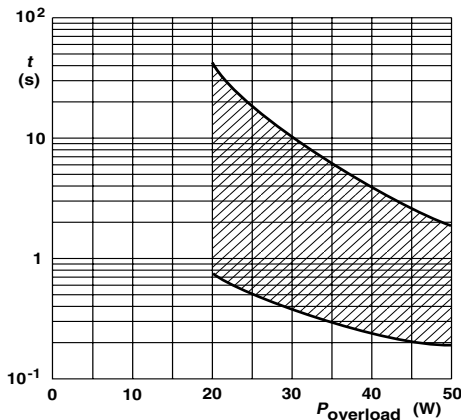
PR01 Time to interruption as a function of overload power for range: 1 R 5 \leq R_n \leq 15 R
