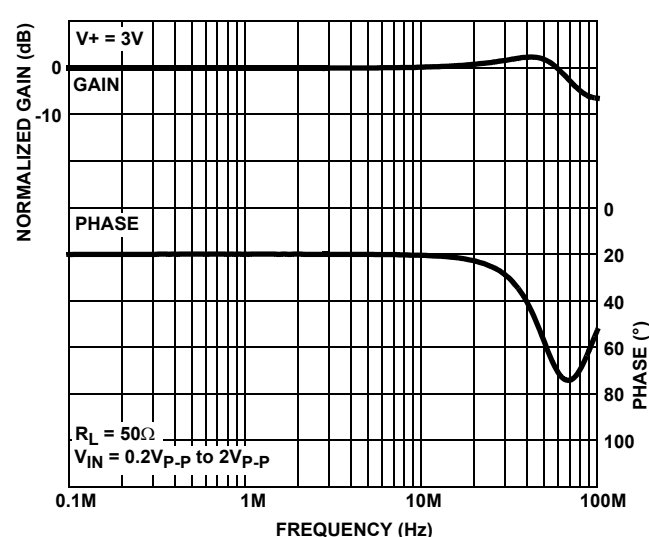
FIGURE 19. FREQUENCY RESPONSE
