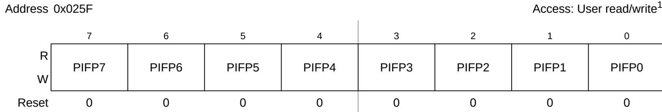
Figure 2-47. Port P Interrupt Flag Register (PIFP)
