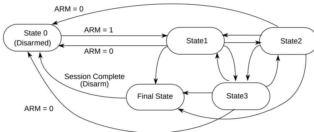
Figure 6-22. State Sequencer Diagram
