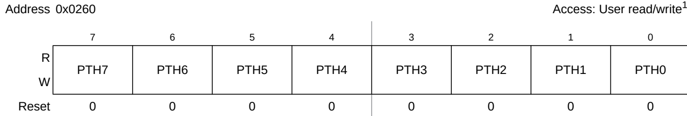
Figure 2-48. Port H Data Register (PTH)
