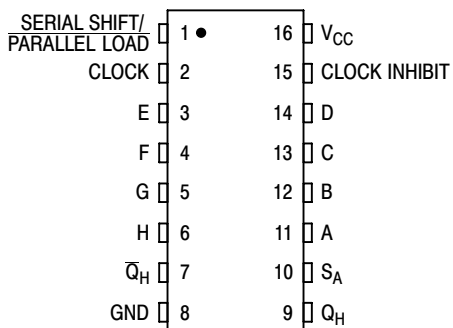
Figure 1. Pin Assignment
