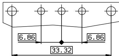
LAYOUT DIMENSIONS (after plating) CONNECTOR SIDE VIEW
