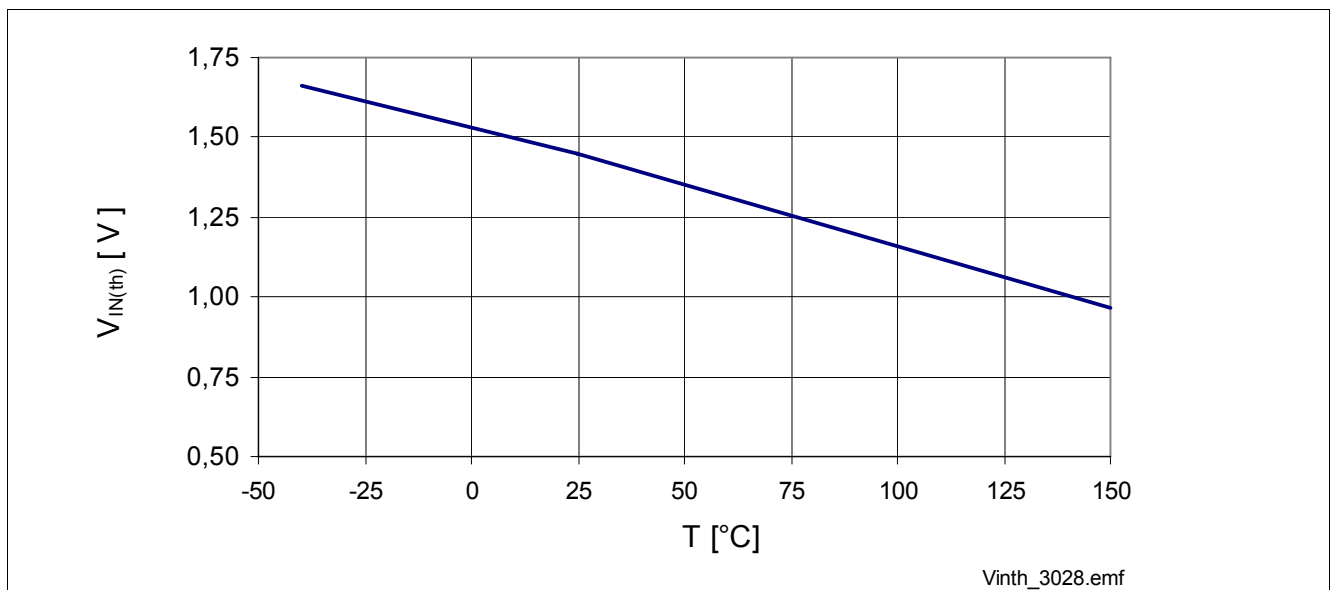
Figure 6 Typical Input Threshold Voltage V_{in} = f(T_J) ; I_D = 1.2mA , V_D = V_{IN}
