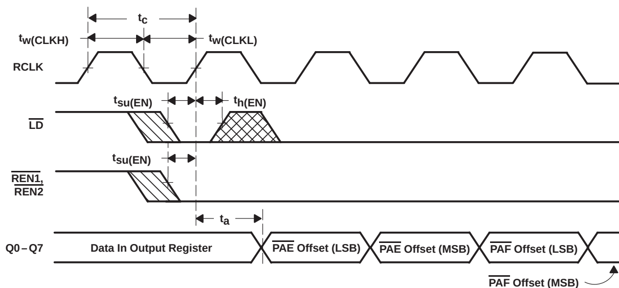
Figure 11. Read-Offset-Registers Timing
