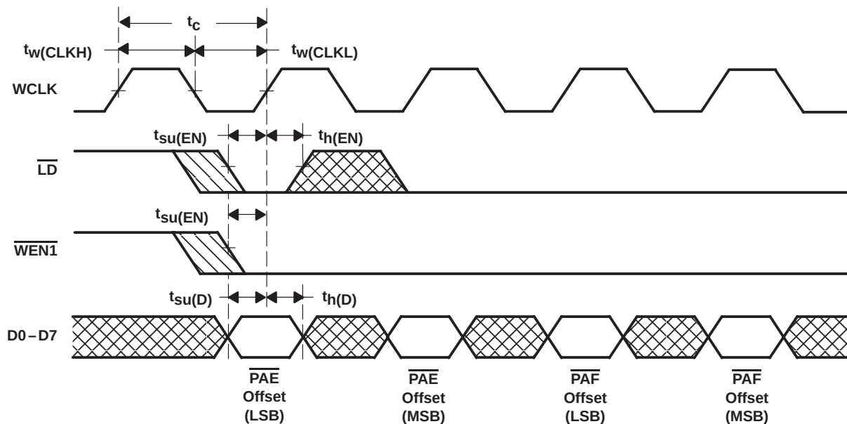
Figure 10. Write-Offset-Registers Timing
