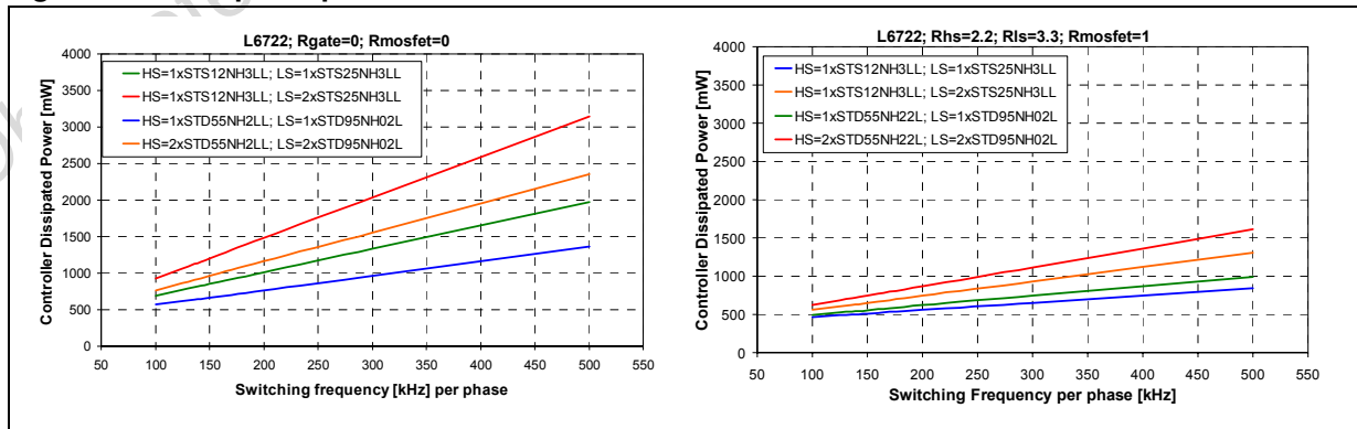
Figure 5. Dissipated power
