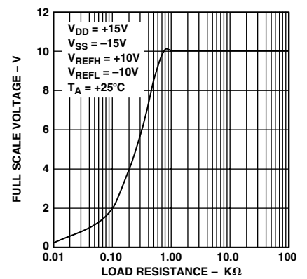
Figure 25. DAC 8412 Output Swing vs. Load Resistance
