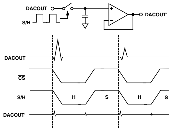
Figure 34. Deglitcher Circuit
