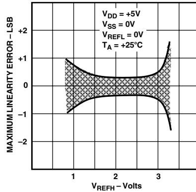
Figure 8. DNL vs. V_{REFH}
