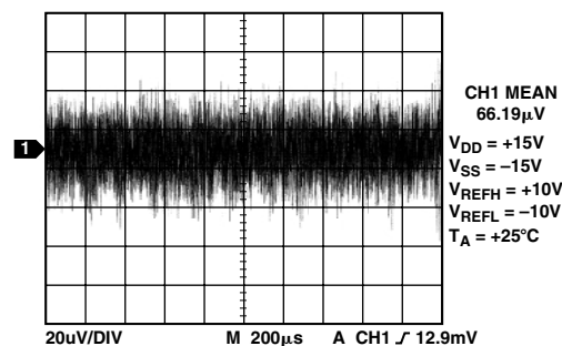
Figure 31. Broadband Noise
