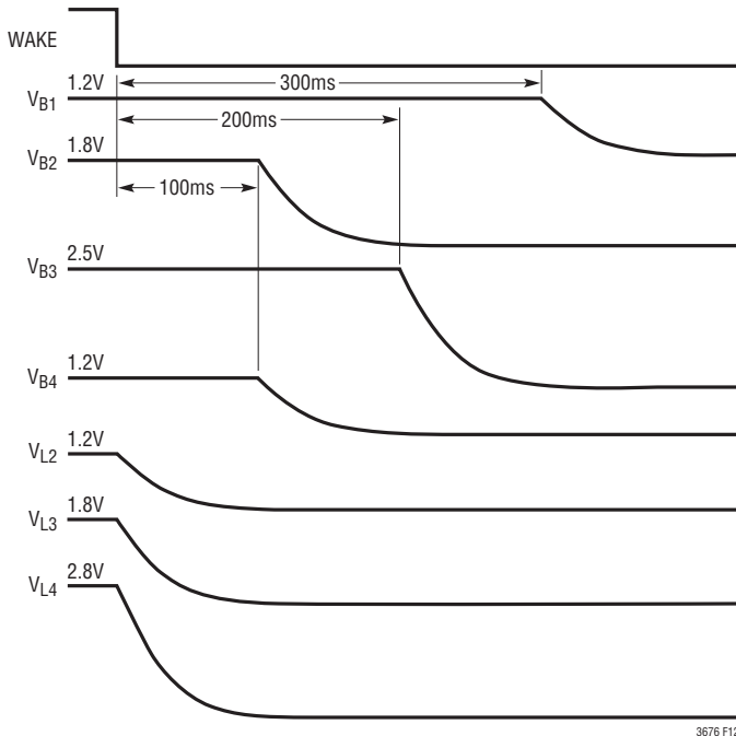
Figure 12. Power-Down Sequence
