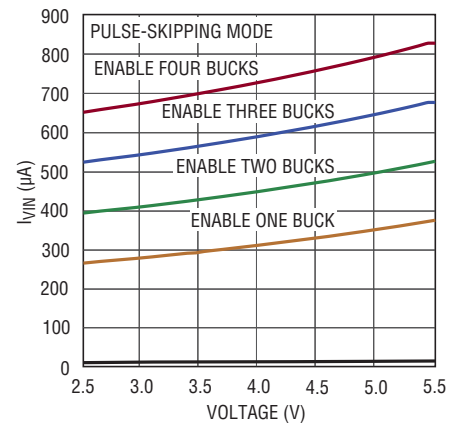
Step-Down Switching Regulator I_{VIN} vs V_{IN}
