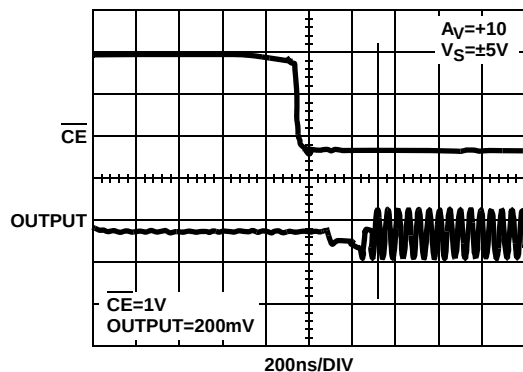
FIGURE 35. ENABLE RESPONSE/TURN-ON TIME
